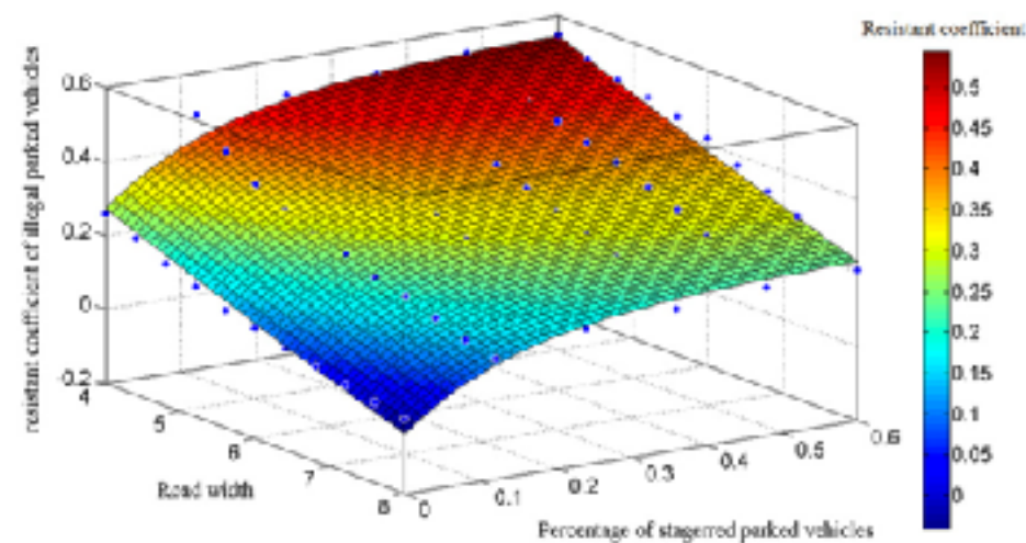
Fig. 6. Relationship of resistant coefficient of illegal vehicle parking, road width and staggered degree of vehicles. (For interpretation of the references to colour in this figure legend, the reader is referred to the web version of this article.)
